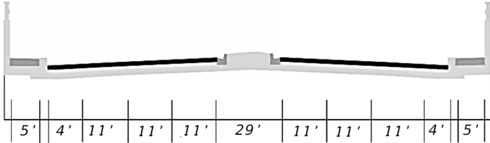
Typical Section 2 (Bridge #860222 over Canal C-14/Cypress Creek)
